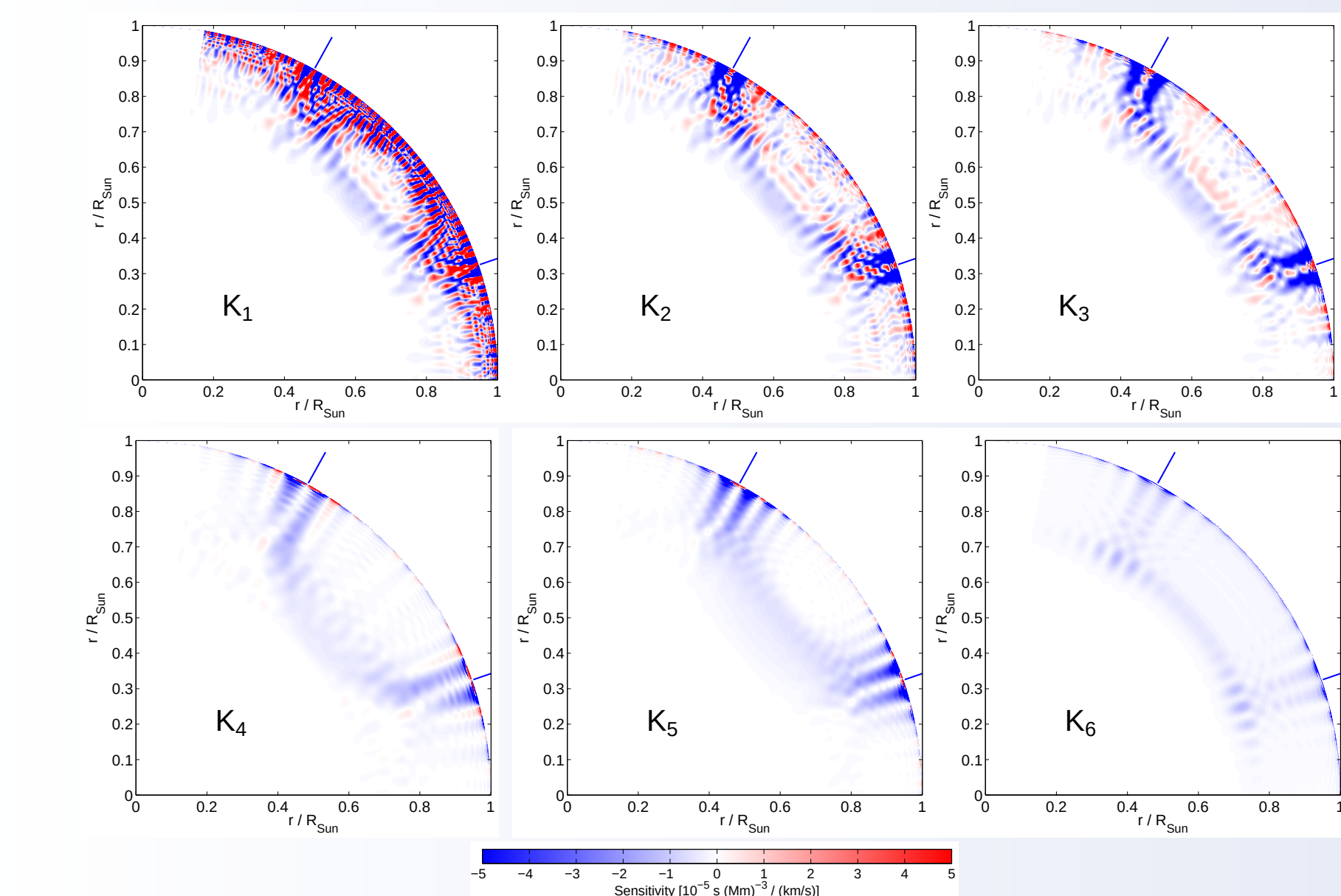
Figure 2: Vertical cuts at the central meridian through example travel-time sensitivity functions for meridional flow, K_\theta , for a travel distance of \Delta = 42^\circ . The locations of the observation points are marked with blue bars.
