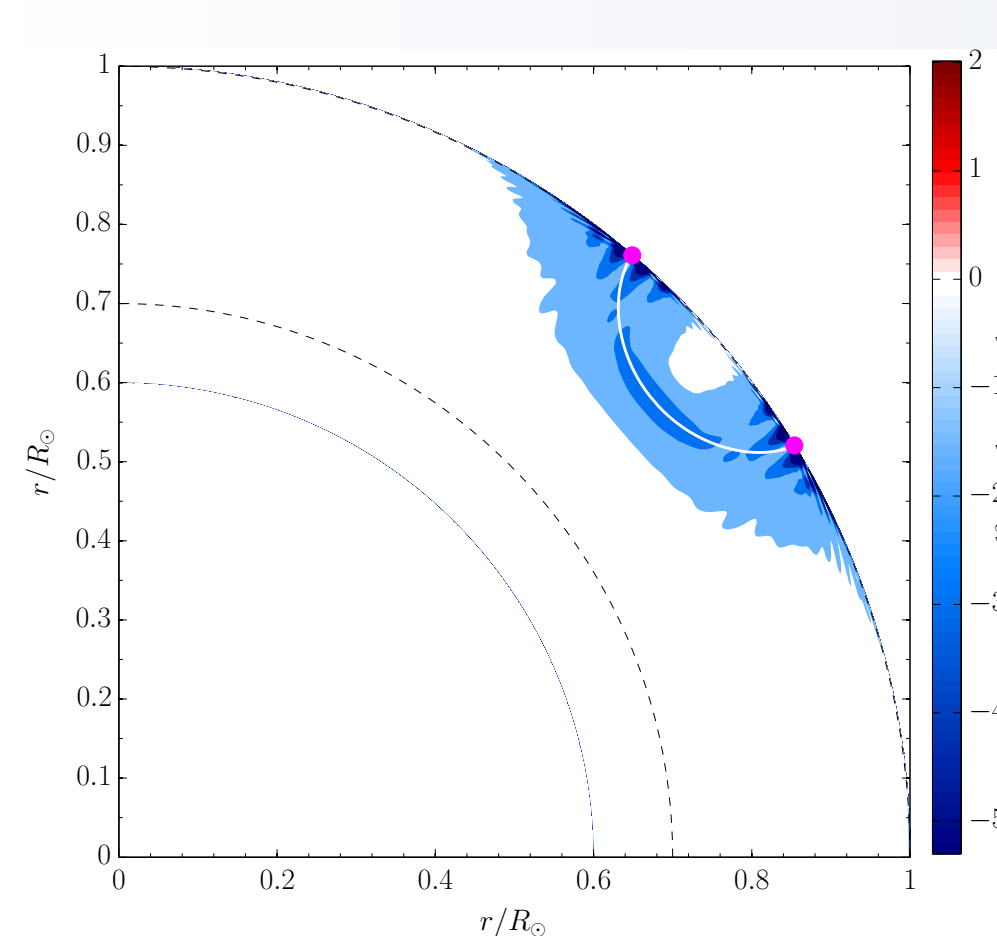
Figure 3: Comparison of Born (shaded 2D-structure) and ray kernels (ray path depicted in white) for an exemplary travel distance of \Delta = 18^\circ .
